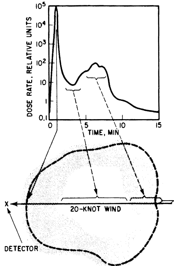
Figure 4-6. Dose Rate vs. Time for a Shallow Underwater Burst
